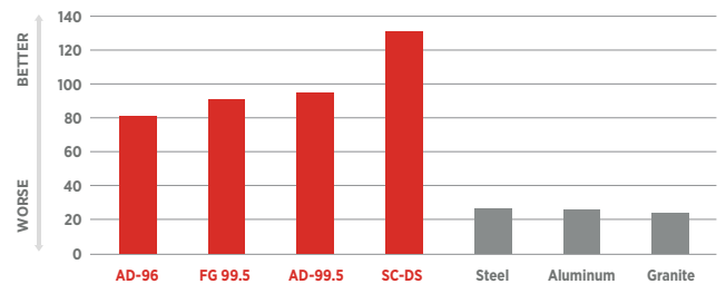
SPECIFIC STIFFNESS (GPa/g/cc)
